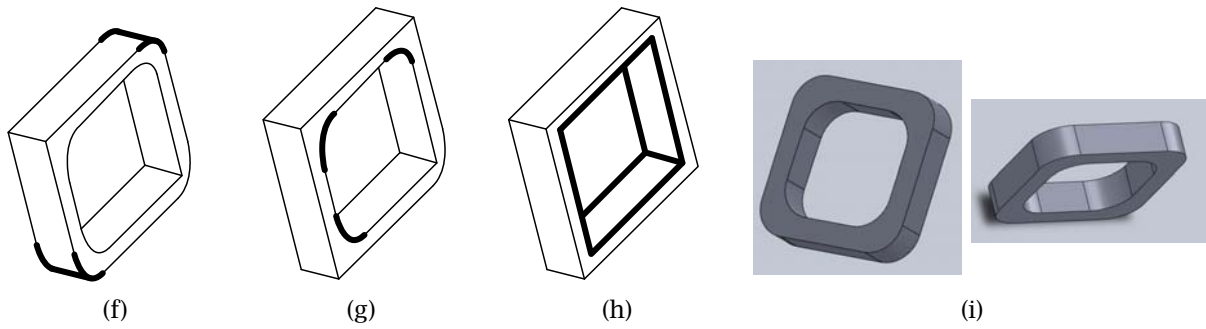
Fig. 6: Example 4: (a) Example 4, (b) Detection of six arcs whose curvatures are the same, (c) Detection of two narrow general fillets, (d) Extraction of the fillets, (e) Detection of two wide general fillets, (f) Extraction of the fillets and detection of two partial fillets, (g) Extraction of the fillets and detection of three hidden fillets, (h) Extraction of the fillets and detection of a rectangular hole, and (i) Two overviews of the solid model in Example 4.
