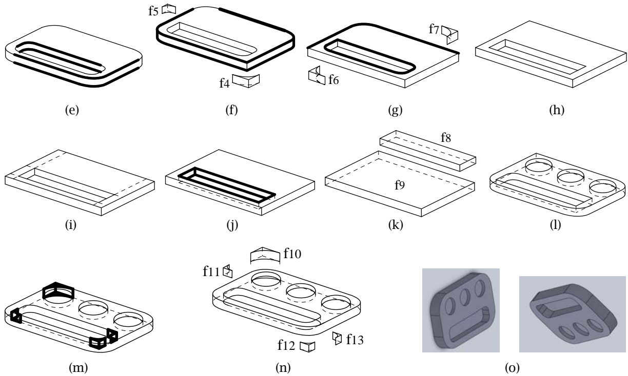
Fig. 5: Example 3: (a) Example 3, (b) Detection of a round hole, (c) Extraction of f_1 , (d) Extraction of f_2 and f_3 , (e) Detection of two general fillets, (f) Extraction of the general fillets and detection of two partial fillets, (g) Extraction of the partial fillets and detection of four hidden fillets, (h) Extraction of the hidden fillets, (i) Drawing of additional lines, (j) Detection of a rectangular hole, (k) Extraction of the hole and detection of a cuboid, (l) Combination of all extracted 3D features except hidden fillets, (m) Recognition of four 3D hidden fillets, (n) Extraction of the fillets, and (o) Two overviews of the solid model in Example 3.
