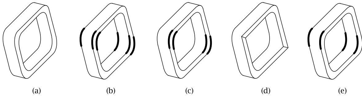
Fig. 5: Example 3: (a) Example 3, (b) Detection of a round hole, (c) Extraction of f_1 , (d) Extraction of f_2 and f_3 , (e) Detection of two general fillets, (f) Extraction of the general fillets and detection of two partial fillets, (g) Extraction of the partial fillets and detection of four hidden fillets, (h) Extraction of the hidden fillets, (i) Drawing of additional lines, (j) Detection of a rectangular hole, (k) Extraction of the hole and detection of a cuboid, (l) Combination of all extracted 3D features except hidden fillets, (m) Recognition of four 3D hidden fillets, (n) Extraction of the fillets, and (o) Two overviews of the solid model in Example 3.
