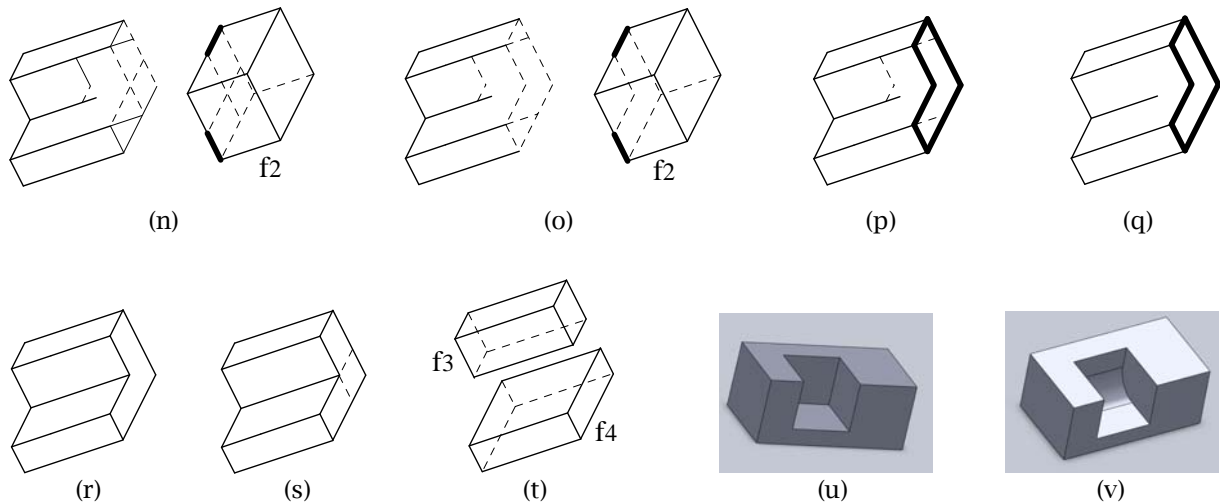
Fig. 8: Example 6: (a) Example 6, (b) Detection of a hidden fillet, (c) Extraction of the fillet and drawing of additional lines, (d) Detection of a cuboid, (e) Removal of the cuboid, (f) Recognition of two contact faces and five contact lines, (g) Change of the contact lines into solid lines, (h) Removal of additional lines of T junctions, (i) Restoration of an isolated solid line, (j) Drawing of additional lines, (k) Detection of another cuboid, (l) Removal of the cuboid, (m) Recognition of four contact edges and six contact lines, (n) Generation of two contact faces, (o) Connection of the two contact faces into a contact face, (p) Change of contact lines into solid lines, (q) Appearance of an isolated solid line, (r) Restoration of the line, (s) Drawing of additional lines, (t) Extraction of f3 and f4, (u) Combination of extracted features except the hidden fillet, (v) An overview of the solid model in Example 6.
